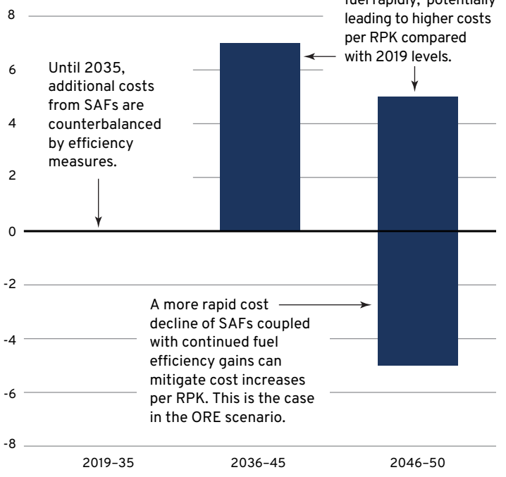
Indicative cost increase per RPK, percentage, compared with 2019 baseline
