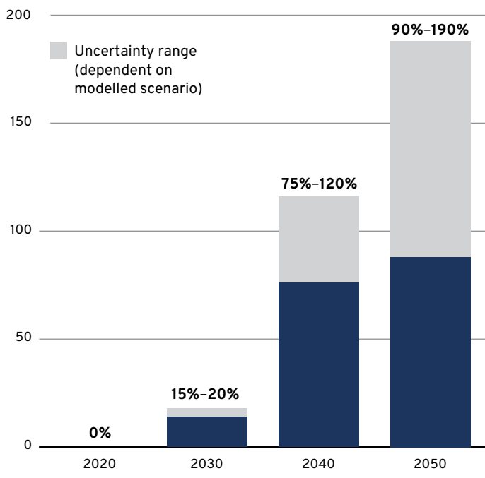
Average aviation fuel cost increase compared with fossil jet fuel costs, %
